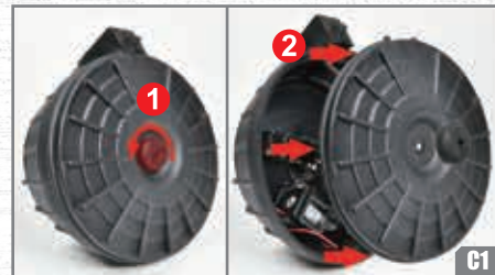
Losen the fixing screw to open the butt plate.
