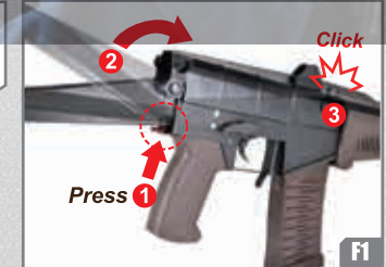
Press the stock release button. Fold the stock to the top of receiver until it's locked.
