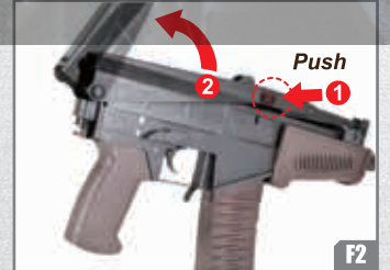
Push back the stock release button. Unfold the stock until it's locked.
