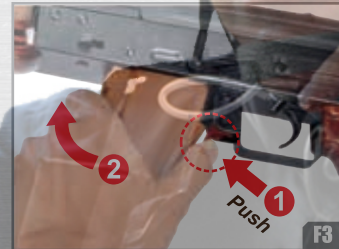
Hold the magazine, push the magazine release lever(step 1) for unloading.
