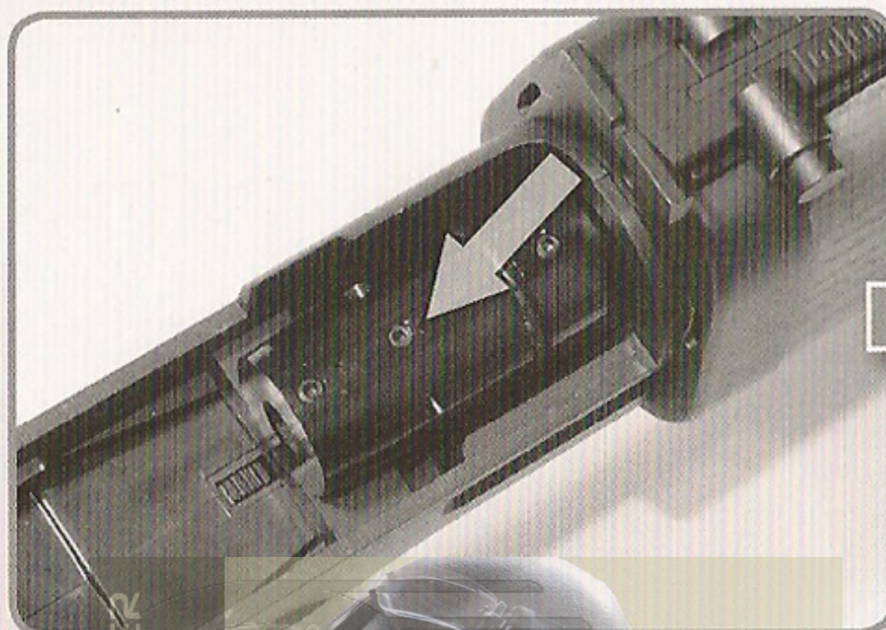
This is the HOP-UP Adjust Screw.
