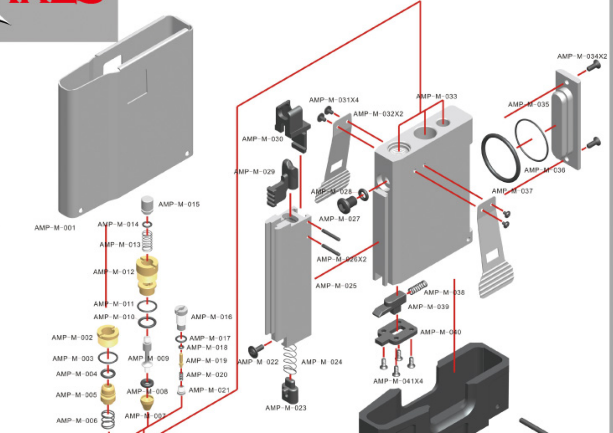
MAGAZINE
