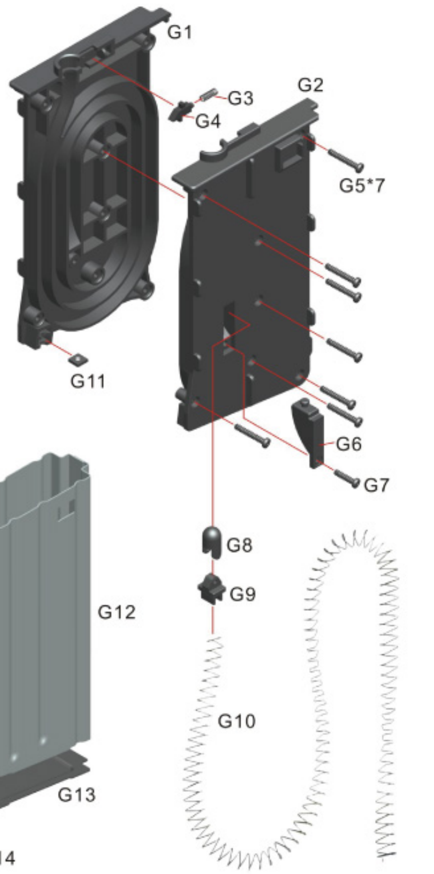
MAGAZINE
