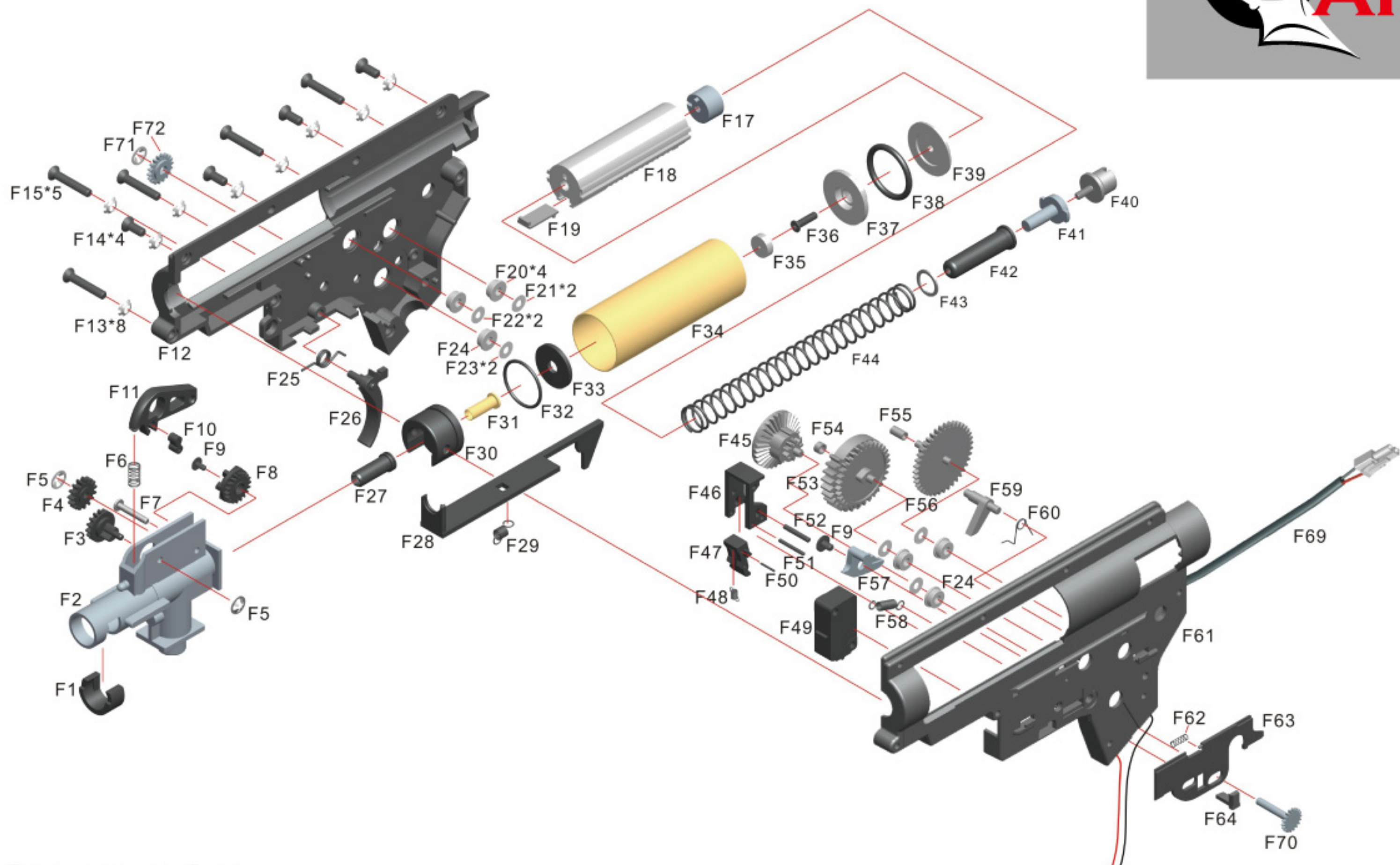
GEARBOX
