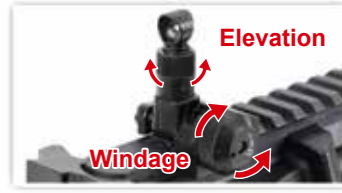
Windage knob (left / right adjustment) Elevation knob (up / down adjustment)
