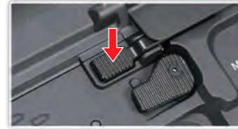
Release the dummy bolt by pressing the bolt release button before closing the eject port cover.
