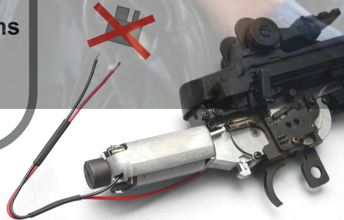
Assemble the butt tube through wires
