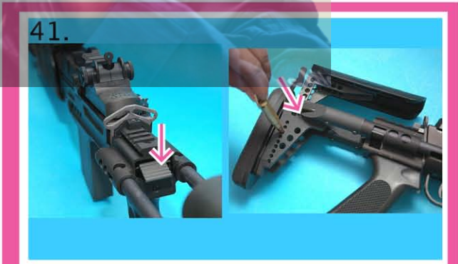
41) 按下解除尾柄鎖及調教面枕 Press down to release collapsible buttstock lock. Cheek piece adjustment
