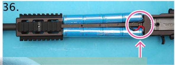
36) 拆除螺絲，安裝電池 Remove screw and forward hand cover to install battery
