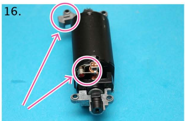
16) 留意部件方向 Pay attention the highlighted parts
