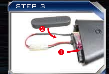
Insert battery then close the butt plate.
