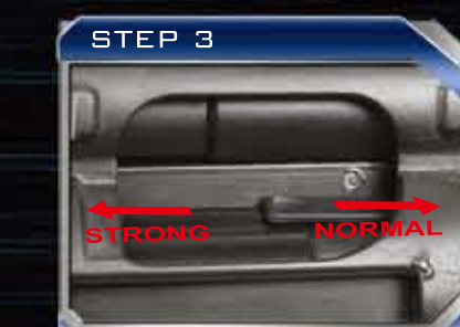
Sliding the Hop-up adjustment piece forward or backward to change the hop-up effect.
