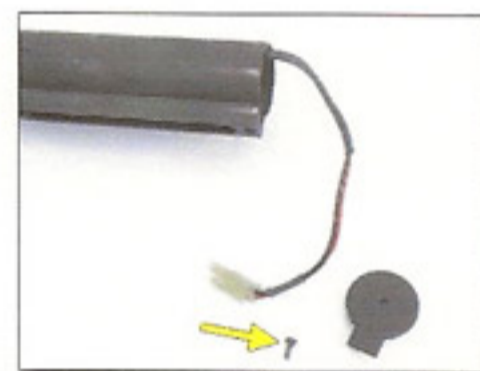
2. Loose the pipe cover screw and remove pipe cover; pull out the wires in the pipe.
