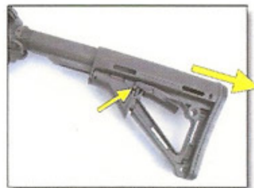
1. In order to install battery to AEG, release the lock clip indicated and take the Magpul stock out.
