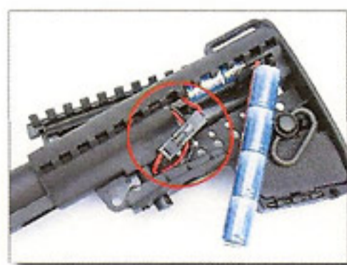
9. Connect the plug as shown. Place the wire and plug inside the stock pipe and make sure the stock can move smoothly.
