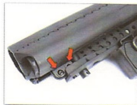
2. Loosen two screws shown.
