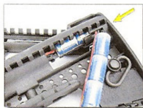
8. Place the single piece battery in the middle of the stock, and put back the stock cover (yellow arrow) to hold the battery on position.
