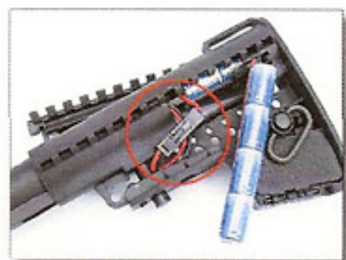
9. Connect the plug as shown. Place the wire and plug inside the stock pipe and make sure the stock can move smoothly.
