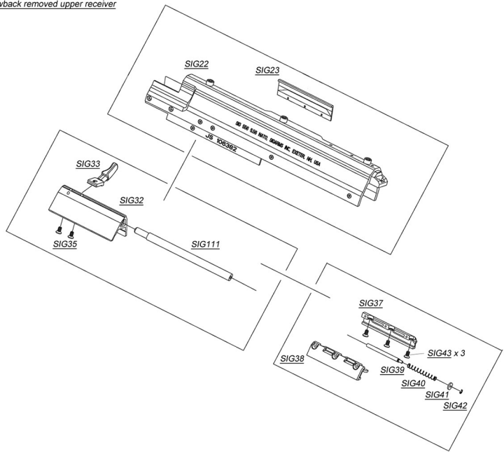
Instruction of blowback removed upper receiver
