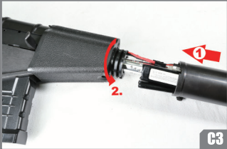
Connect a battery. Attach the handguard by steps.
