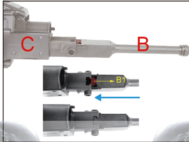
1. 將B1向下壓再依藍箭頭方向組裝至C。 To press B1 downward and toward to C (blue arrow) to assemble.
