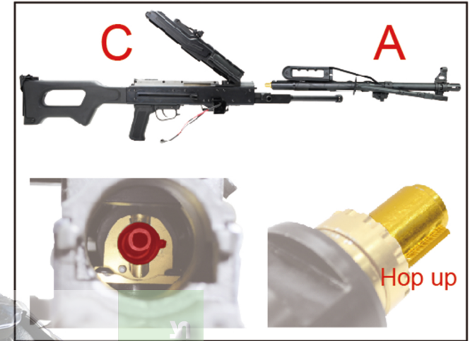
2.A組裝至C，將HOP UP卡榫對齊紅區塊。 To assemble A to C by aligning the HOP UP with red area.
