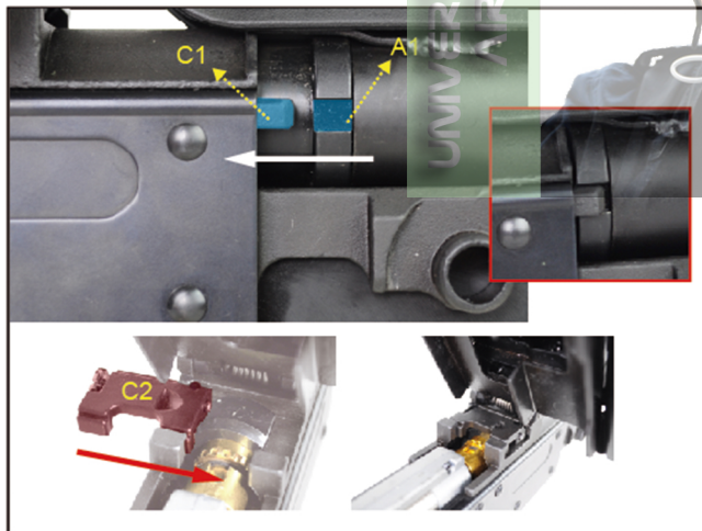
3.A1依白箭頭方向組裝至C1，再將C2往紅箭頭方向移動固定A。 To ensure the A1 be plugged by C1, then move C2 toward red arrow to fix A1.
