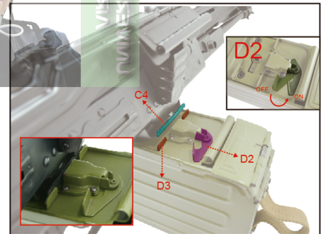
5. 先將D2依紅箭頭方向開啟後，再將C4、D3兩處對齊，關起D2開關即完成組裝。 To turn on D2, align C4 with D3 and turn off D2, then finish to assemble.
