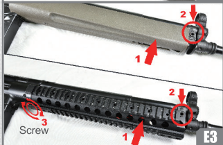
Connect the battery. Attach the handguard by steps.
