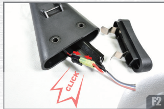
Connect a battery. Attach butt plate by reversed steps.
