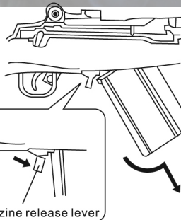
Magazine release lever
