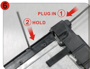
6 將頂彈頭下壓並使之固定 Plug in the follower and hold it.
