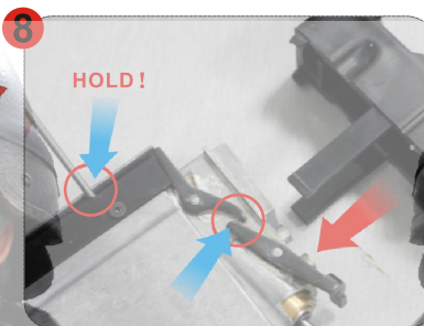
8 組裝新款上蓋前注意箭頭處(頂彈頭)與(卡榫搖臂)的位置 Before assembling the new cover make sure the "follower" and "follower link" is in the right position.
