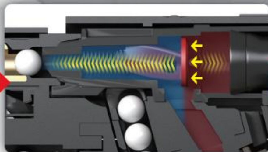
The remaining gas is filled up to the rear part of the cylinder and it pushes the valve forward.
