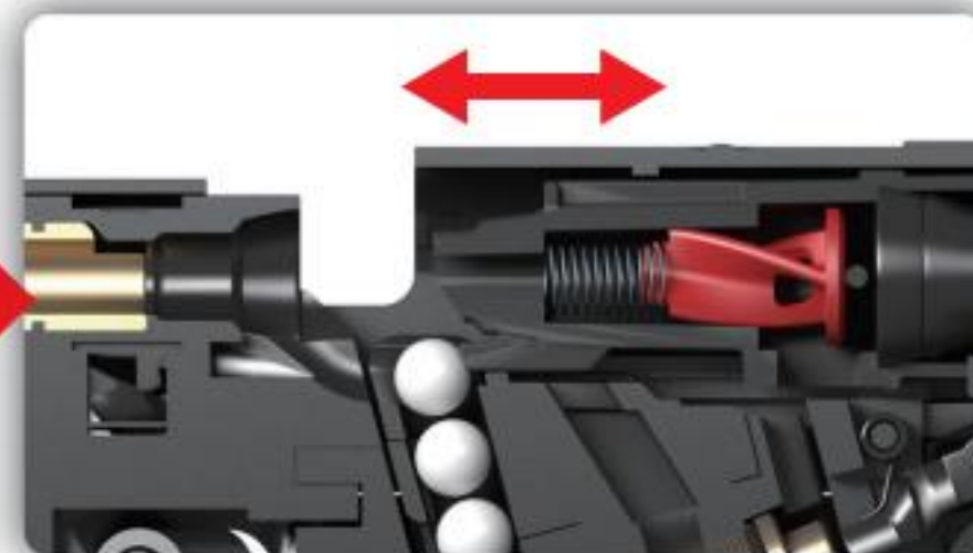
The leftover gas will push the piston and bring the slide backwards.
