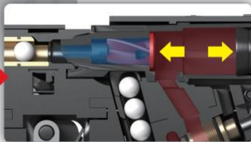
Whirl valve will be pushed until the cylinder is closed.
