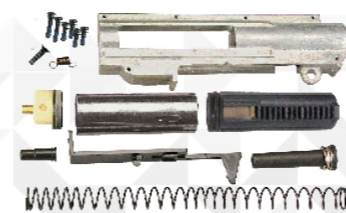
Upgrade Upper Gearbox A (M120 Spring, Plastic Piston) 升級上齒輪箱組 -A (M120 彈簧; 原廠塑膠活塞) MA-47
