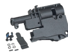
MAR Rear Sight Set MAR 視孔座組 MK-16
