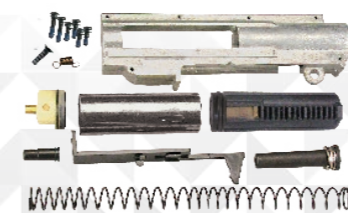
Upgrade Upper Gearbox B (M120 Spring, Aluminum Piston) 升級上齒輪箱組 -B (M120 彈簧; 鋁活塞) MA-48
